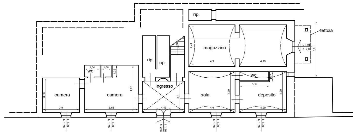
PIANO TERRENO
